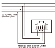
Telephone Outlet - RJ11
