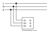
Connection Unit
