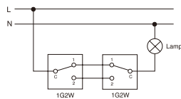
Two-Way Switch
