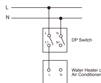
Double-pole One-Way Switch
