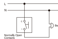
Retractive Switch
