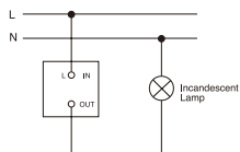
Rotary Dimmer
