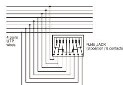
Computer Outlet - RJ45
