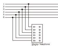
Telephone Outlet - BT
